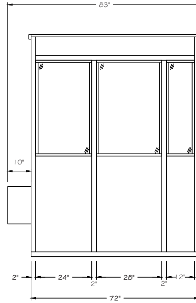
E3 RIGHT ELEVATION SCALE \frac{1}{2}'' = 1' - 0''
