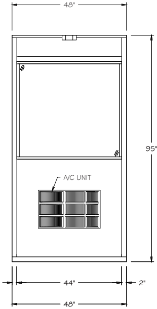
E4 REAR ELEVATION SCALE \frac{1}{2}'' = 1' - 0''
