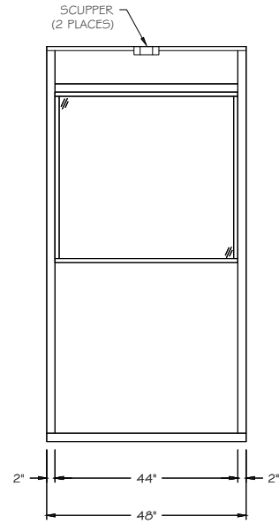
E2 FRONT ELEVATION SCALE \frac{1}{2}'' = 1' - 0''
