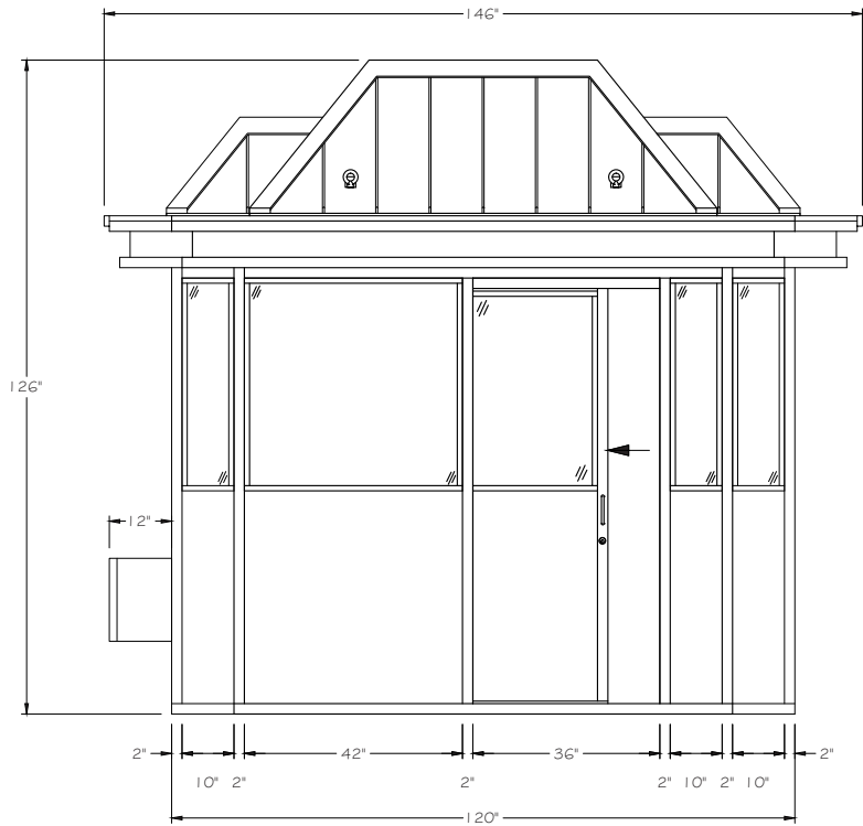
E3 RIGHT ELEVATION SCALE \frac{1}{2}'' = 1'-0''
