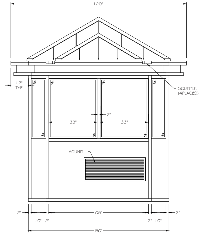
E4 REAR ELEVATION SCALE \frac{1}{2}'' = 1'-0''
