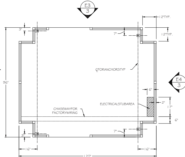
STUB AREA
