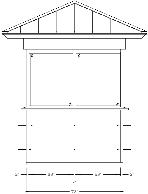
E2 FRONT ELEVATION SCALE \frac{1}{2}'' = 1' - 0''
