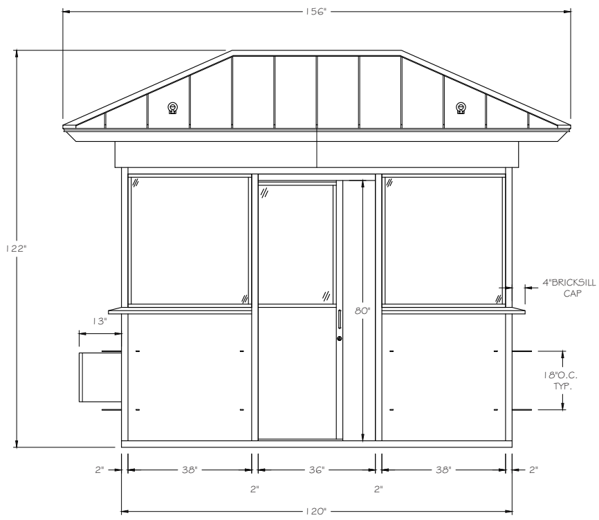
E3 RIGHT ELEVATION SCALE \frac{1}{2}'' = 1'-0''
