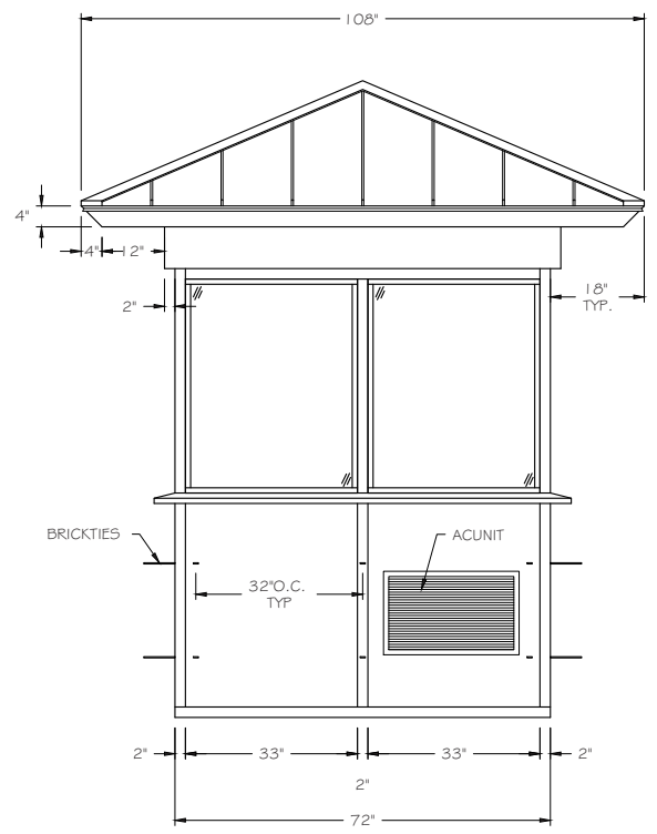
E4 REAR ELEVATION SCALE \frac{1}{2}'' = 1'-0''
