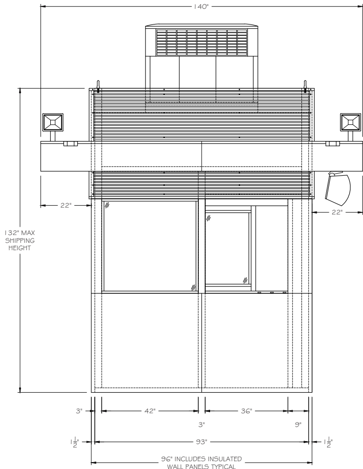
E2 FRONT ELEVATION SCALE \frac{1}{2}'' = 1' - 0''
