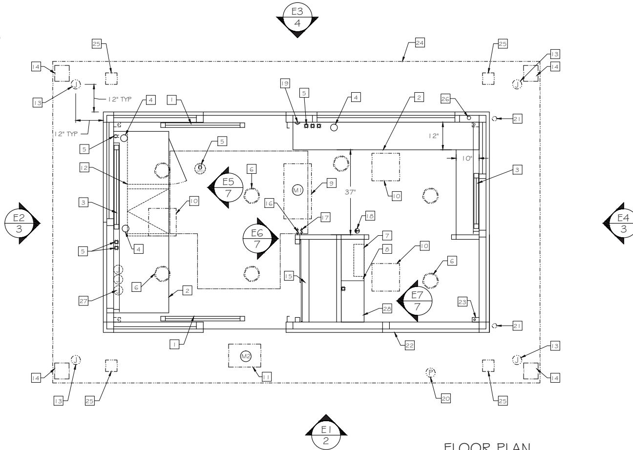
FLOOR PLAN SCALE 1/2" = 1' - 0"
