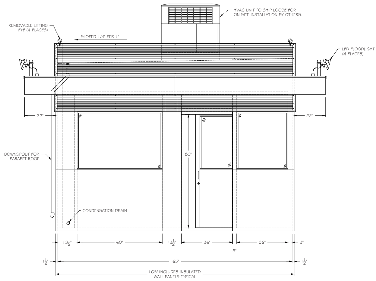
E3 RIGHT ELEVATION SCALE \frac{1}{2}'' = 1' - 0''
