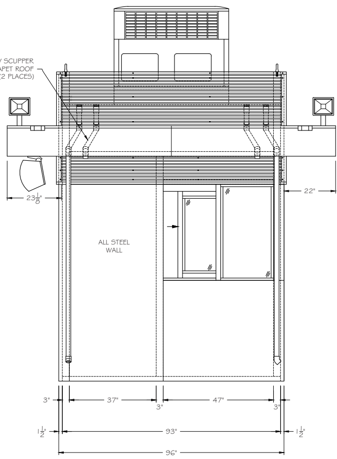
E4 REAR ELEVATION SCALE \frac{1}{2}'' = 1' - 0''
