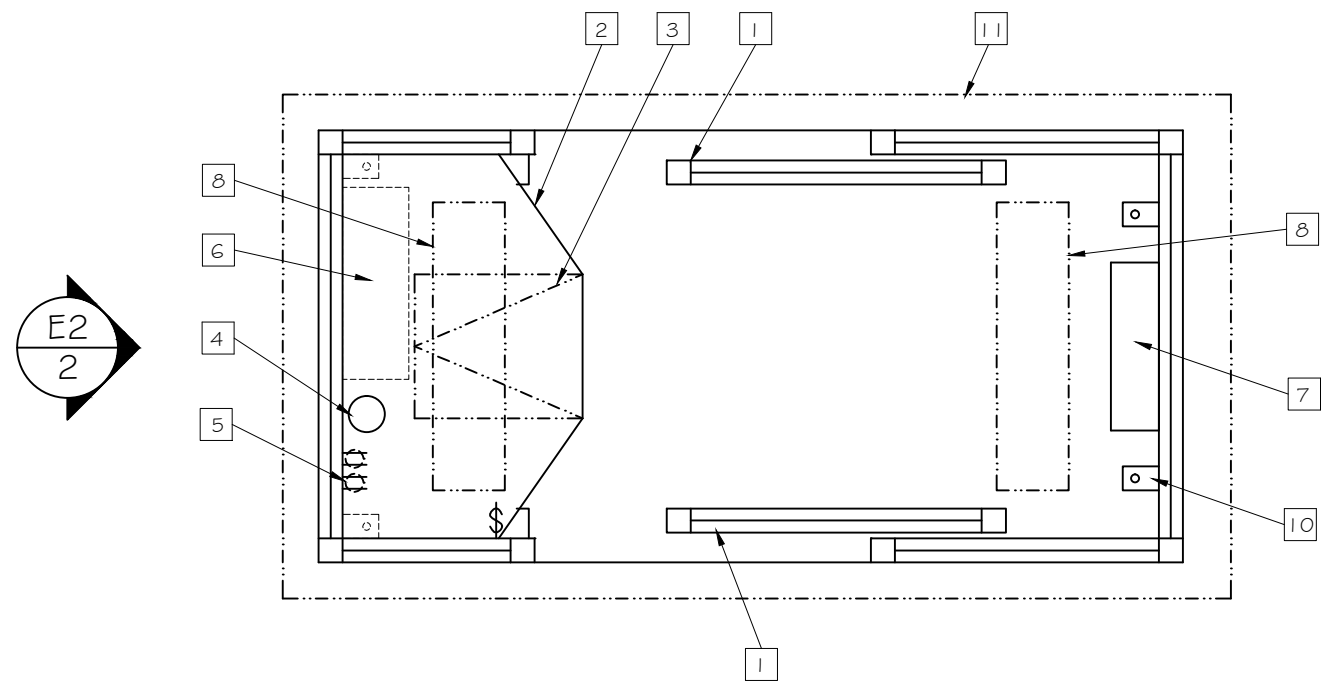
FLOOR PLAN SCALE \frac{3}{4}'' = 1' - 0''
