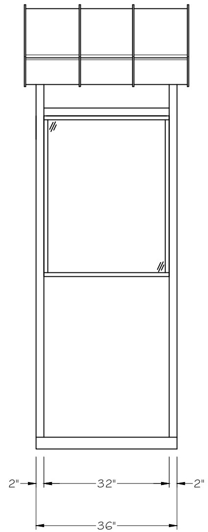
E3 REAR ELEVATION SCALE: \frac{1}{2}'' = 1' - 0''
