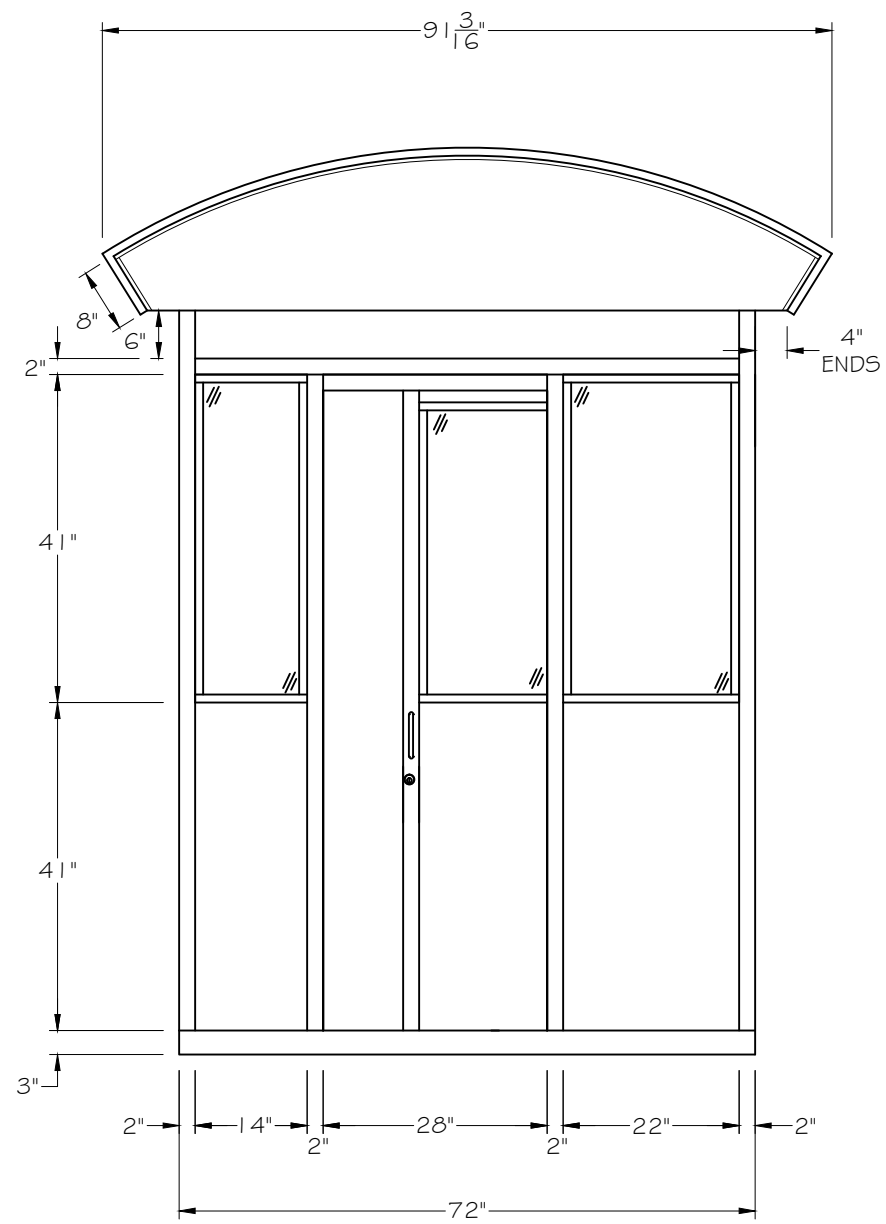
E1 LEFT ELEVATION SCALE: \frac{1}{2}'' = 1' - 0'' RIGHT ELEVATION OPPOSITE
