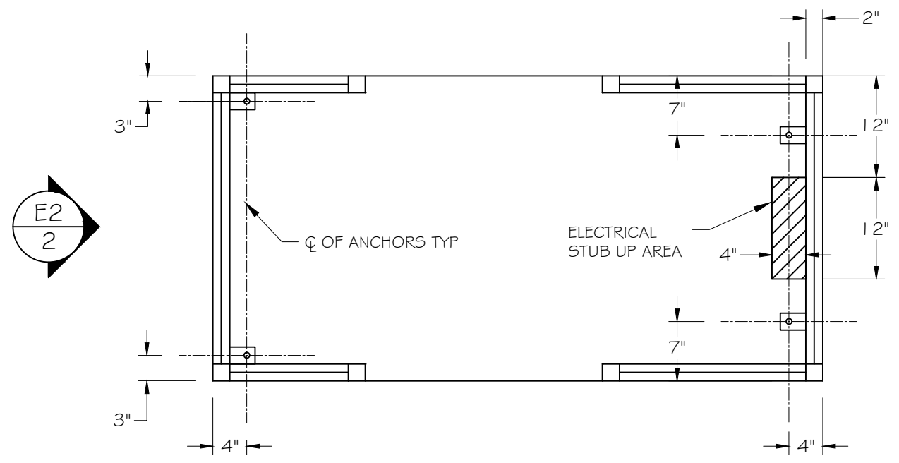
ELECTRICAL STUB AREA PLAN SCALE \frac{3}{4}'' = 1' - 0''
