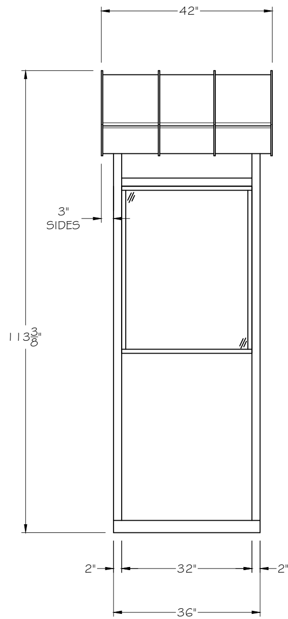
E2 FRONT ELEVATION SCALE: \frac{1}{2}'' = 1' - 0''
