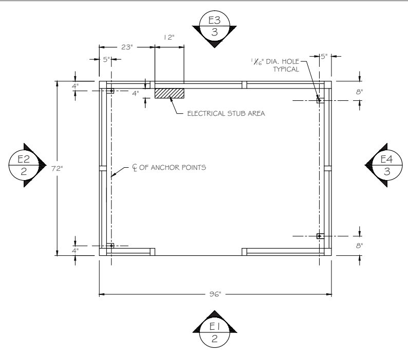
STUB UP AREA & ANCHOR LOCATIONS SCALE \frac{1}{2}'' = 1' - 0''
