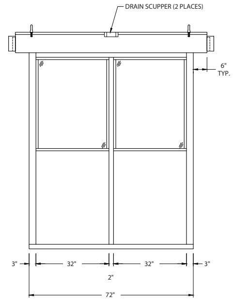
E2 FRONT ELEVATION SCALE \frac{1}{2}'' = 1' - 0''
